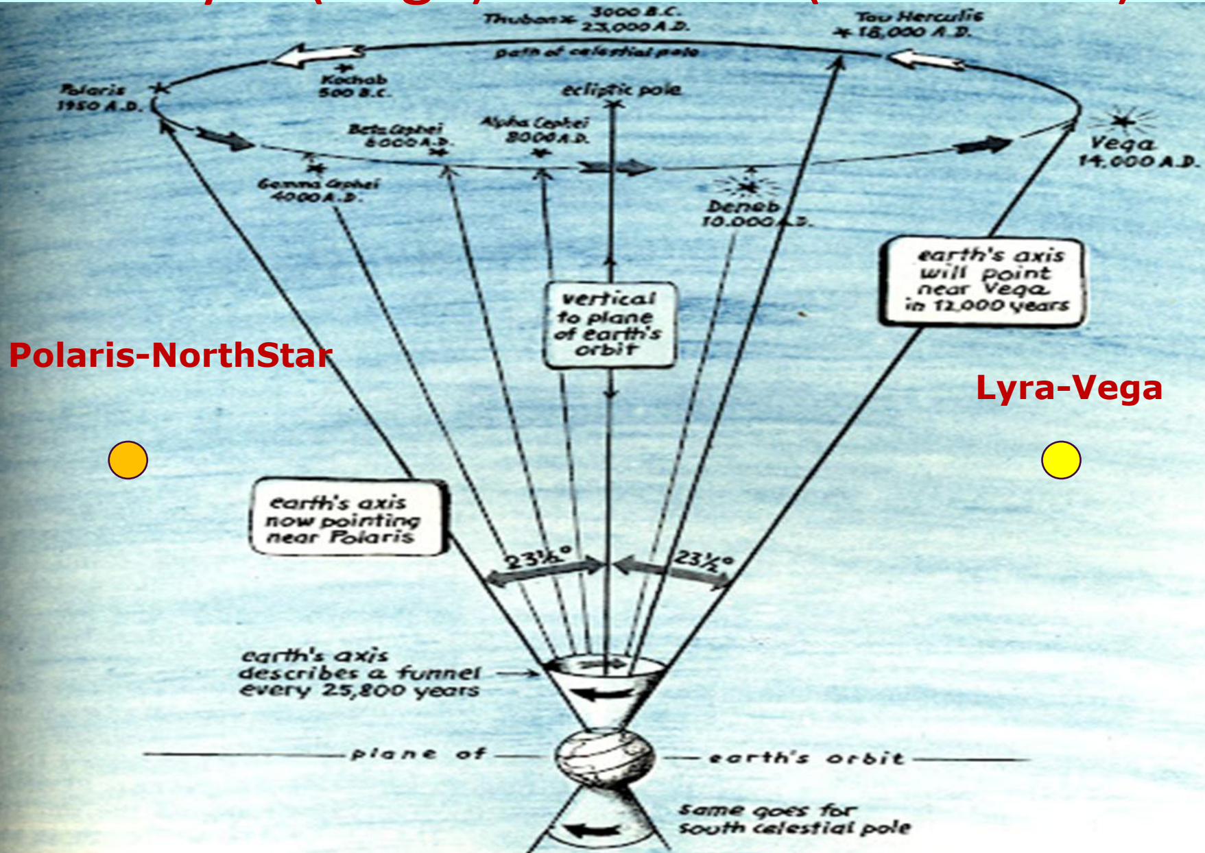
Figure 24: The Wobble of the Earth's Axis
